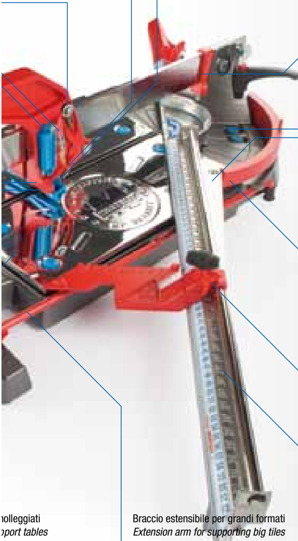
Rotella di incisione a vista titanium gold High visibility of incision wheel
